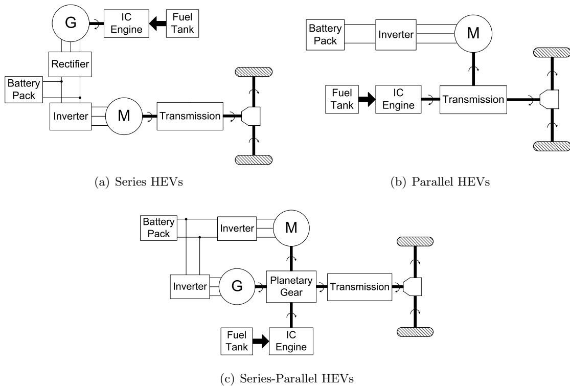
Figure 2.1 HEV Configurations.
